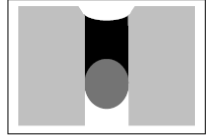
The recessed joint design projects the sealant against mechanical loads.
